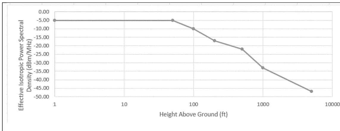
Figure 1 to Paragraph (g)(1)(i)—Fundamental Effective Isotropic PSD at Outside Interface of Aircraft Antenna
